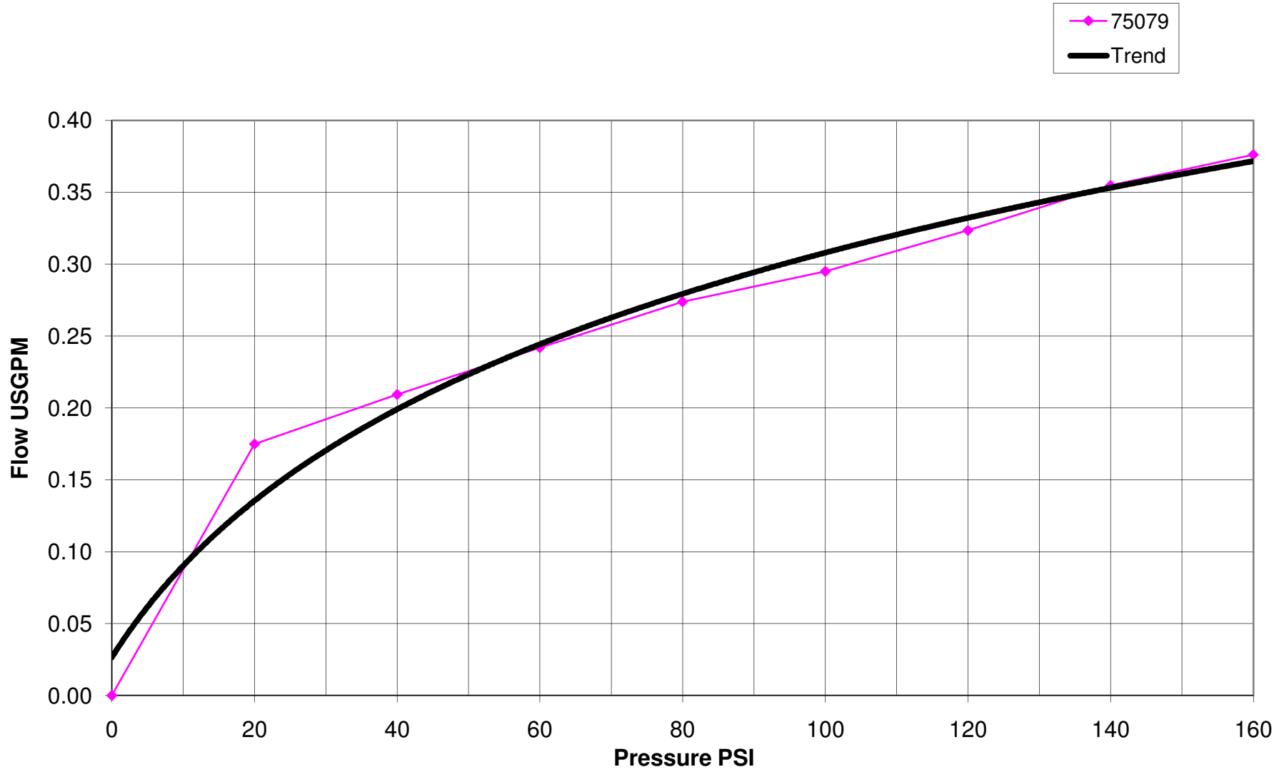
Flow Chart for 75079 1.0mm Orifice J30 Spray in USGPM
